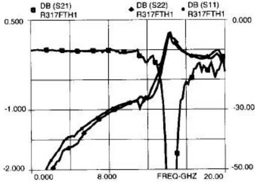
Figure 5. Feedthrough Frequency Response
