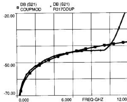
Figure 9. Package Isolation
