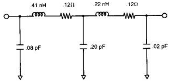
Figure 7. Feedthrough Model
