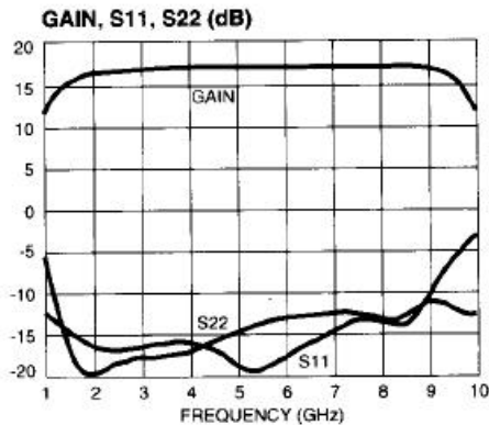
Figure 6. MAAM28000-A1 Performance
