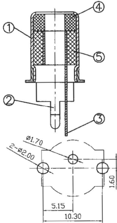
Pin Hole Layout (Jack Bottom View)
