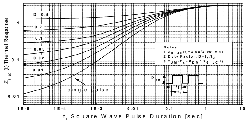
Transient Thermal Response Curve For JCS5N50FT
