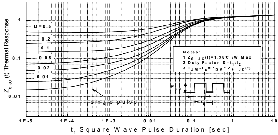
Transient Thermal Response Curve For JCS5N50CT
