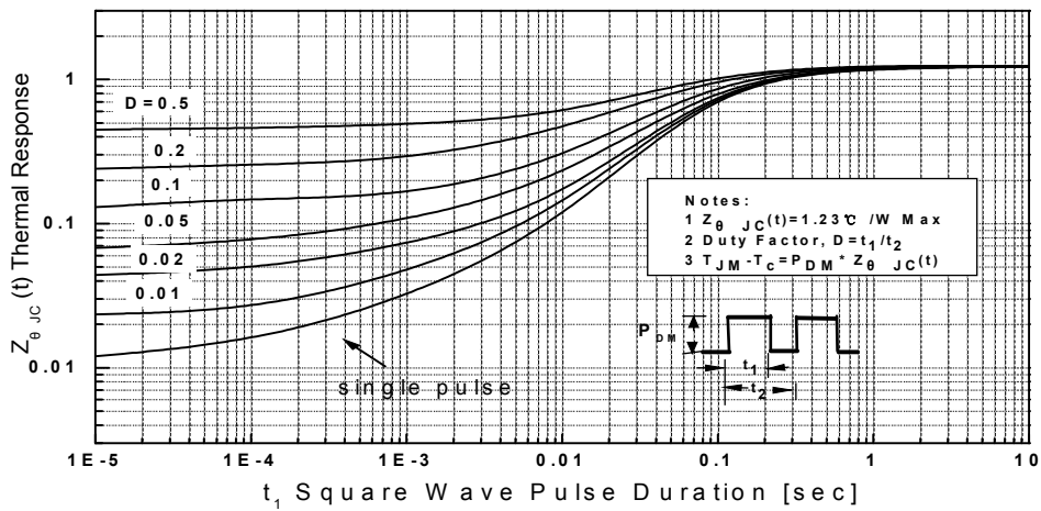
Transient Thermal Response Curve For JCS5N50FT
