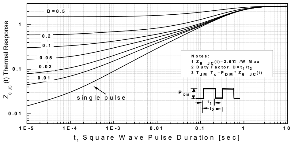
Transient Thermal Response Curve For JCS9N50FT
