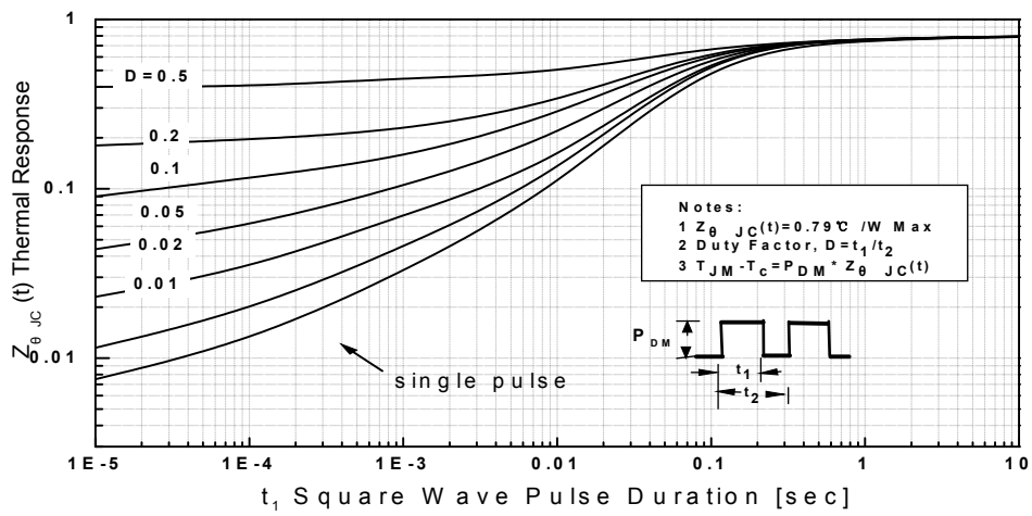
Transient Thermal Response Curve For JCS9N50CT
