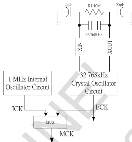
Figure 5-2 FS98023 oscillator state block
