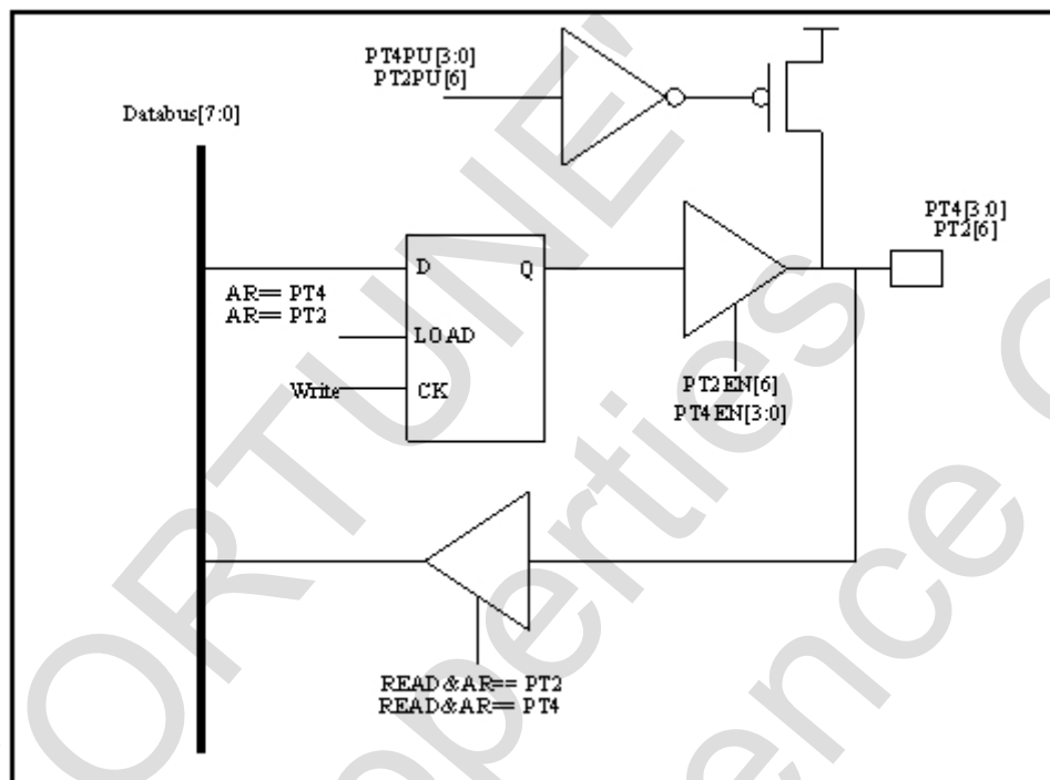
Figure 7-5 PT2[6] and PT4[3:0] function block
