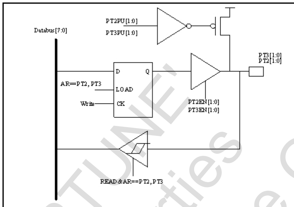
Figure 7-2 PT2[0], PT2[1], PT3[0], PT3[1] function block
