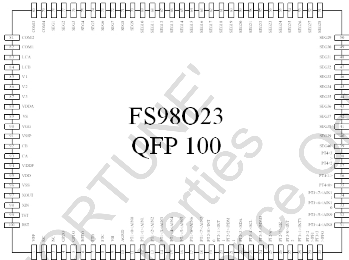
Figure 1-1 FS98023 pin configuration
