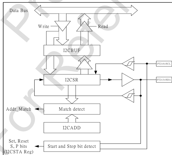
Figure 9-2 I2C module function block
