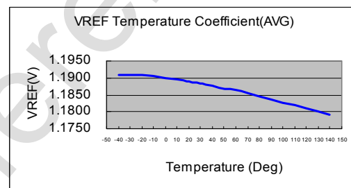
Figure 2-2 VREF vs Temp @ VDD=3V
