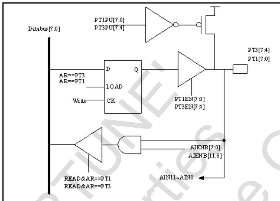
Figure 7-1 PT1[7:0] function block
