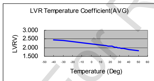
Figure 2-3 LVR vs Temp @ VDD=3V
