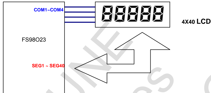
Figure 13-1 LCD driver control block
