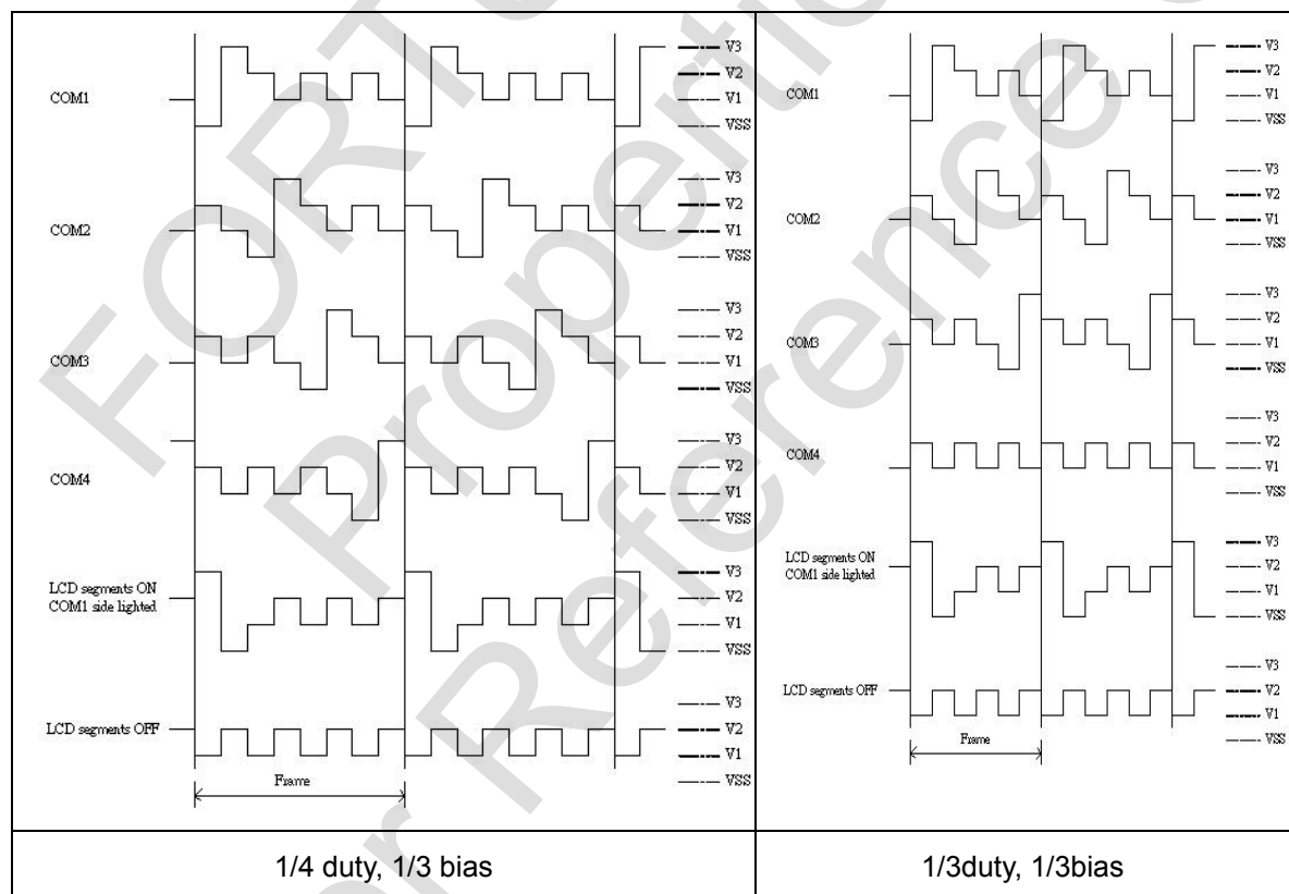
Figure 13-5 1/3 bias LCD power system clock
