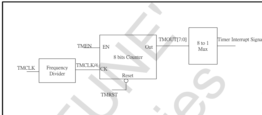
Figure 6-1 FS98023 timer module function block
