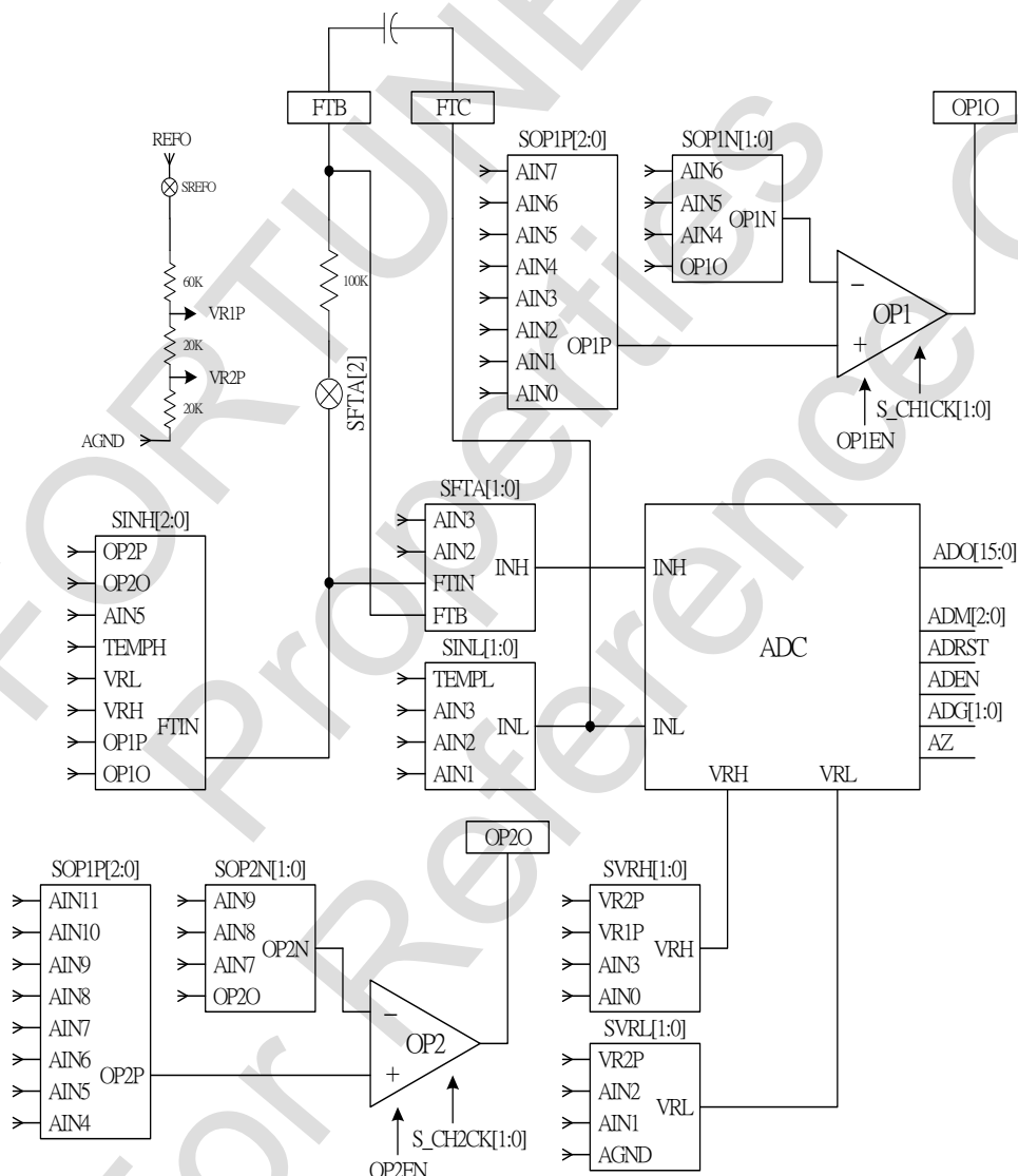
Figure 10-1 FS98O23 analog function network
