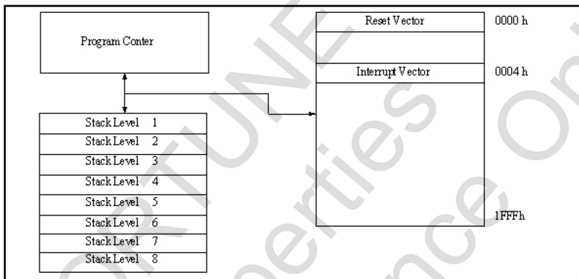
Figure 3-1 FS98023 program memory structure
