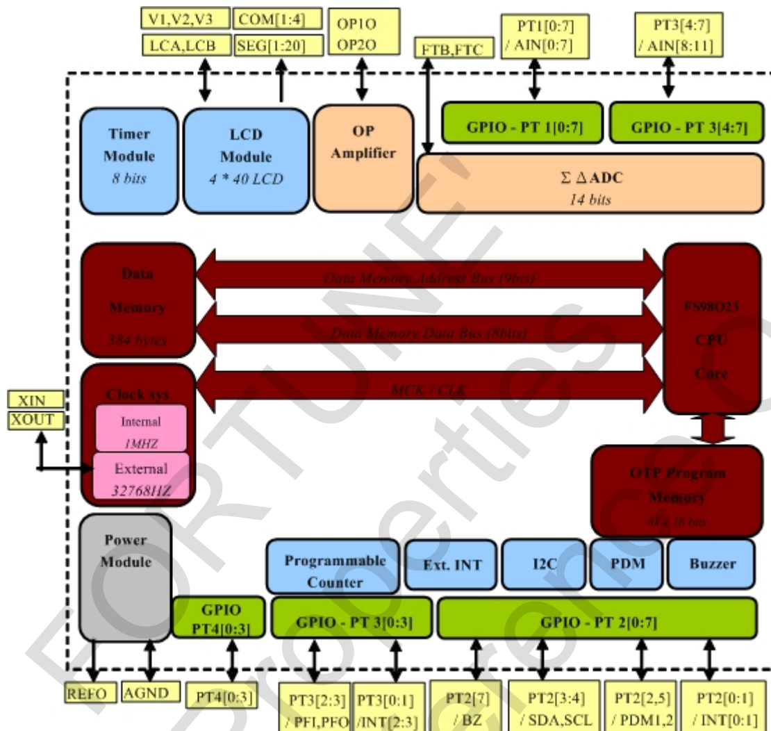
Figure 1-2 FS98023 function block
