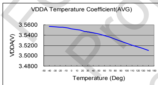
Figure 2-1 VDDA vs Temp @ VDD=3V
