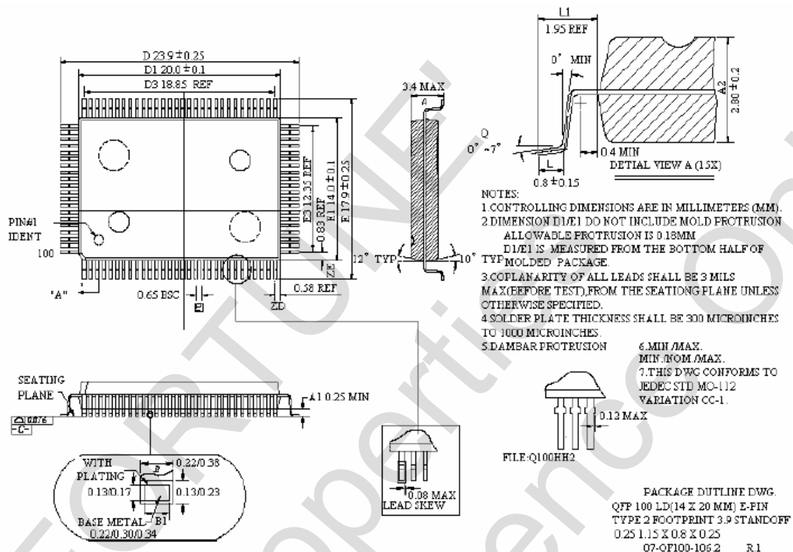
Figure 16-1 FS98O23 package outline
