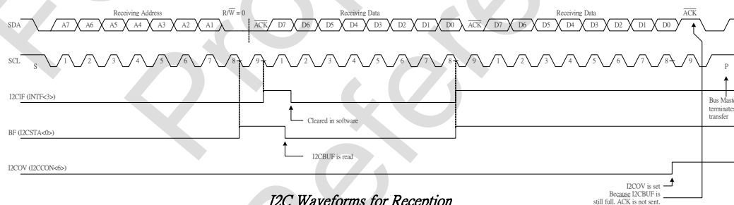
I2C Waveforms for Reception
