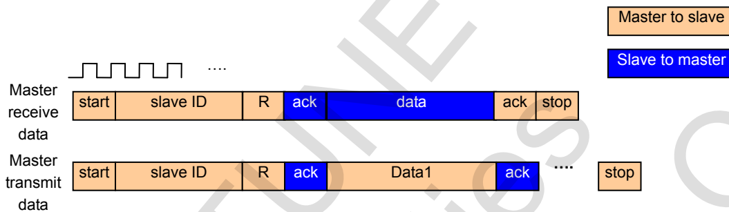
Figure 9-1 FS98023 I2C module communication
