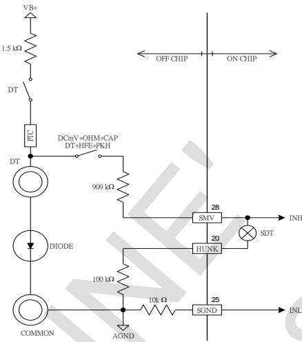
Graph 25. Function network of diode measurement.
