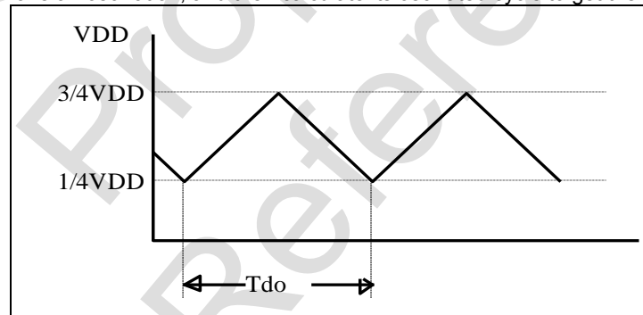
Capacitor Measurement
