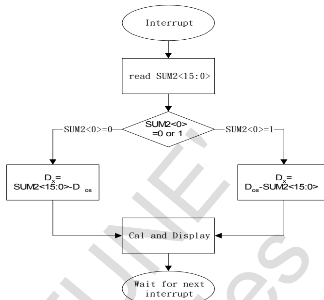
Graph 13. The flow-Chart of operation and display of fast ADC output.
