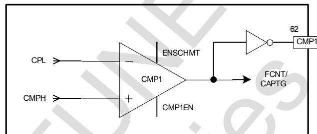
Graph 8. Comparator Block-diagram.
