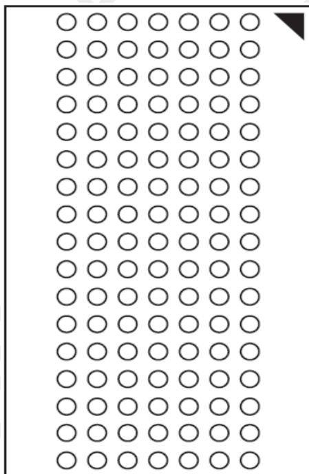
Bottom View 119-Ball, 14 mm x 22 mm BGA 1 mm Ball Pitch, 7 x 17 Ball Array
