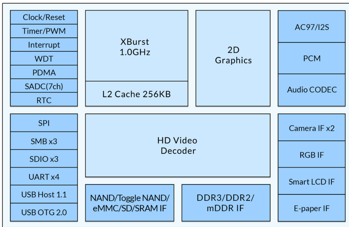
Figure 1-1 JZ4775 Diagram
