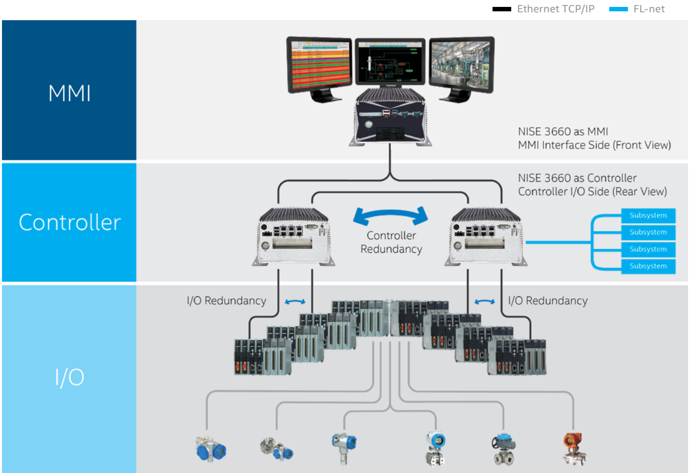
NEXCOM NISE 3660 as deployed in the customer's DCS
