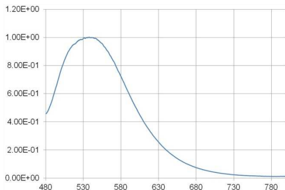
Emission Spectrum
