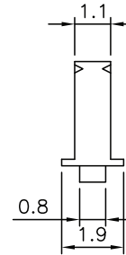
C-C SEC
