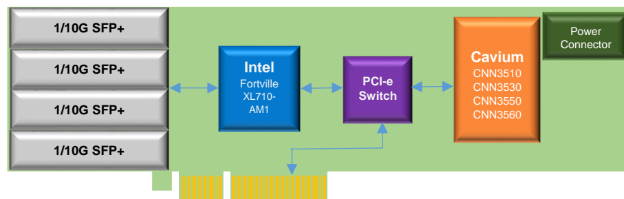
Block Diagram of Sierra 3351
