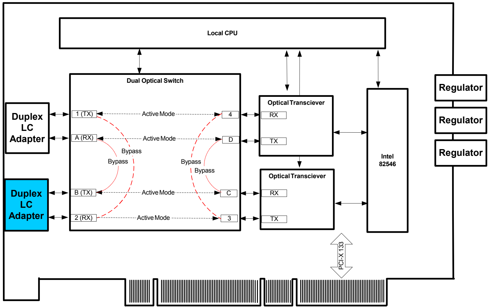
Figure 1 Block Diagram
