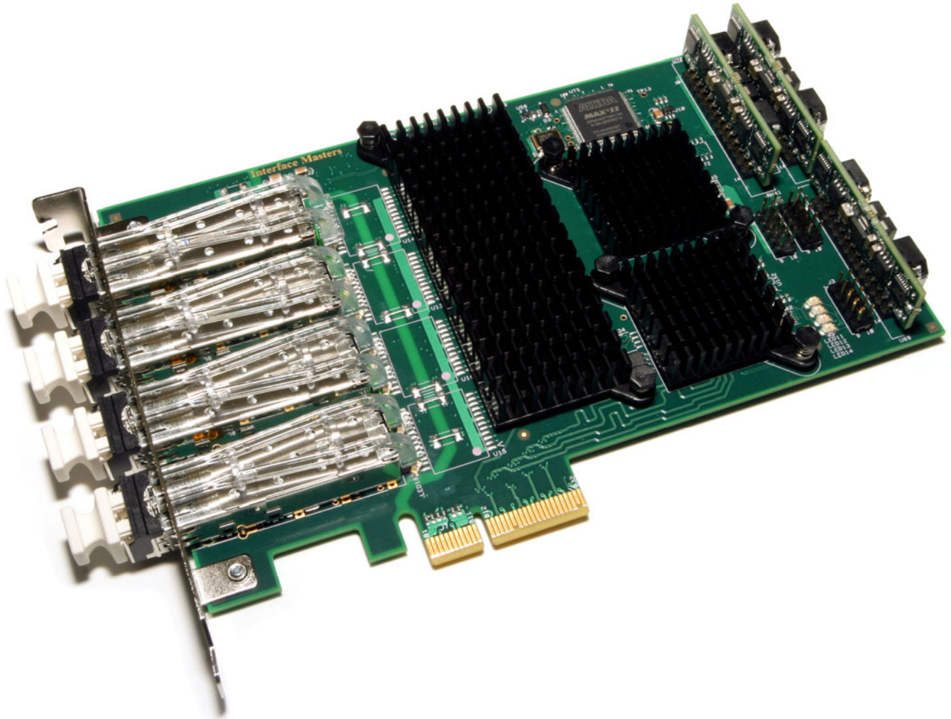
Figure 1, Niagara 2384, Quad Giga bit NIC with SFP & Cavium CN16XX
