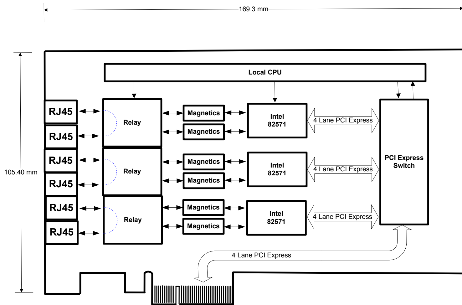
Figure 1 Block Diagram
