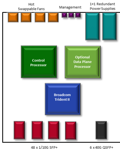
Niagara 2948X6XL Functional Block Diagram
