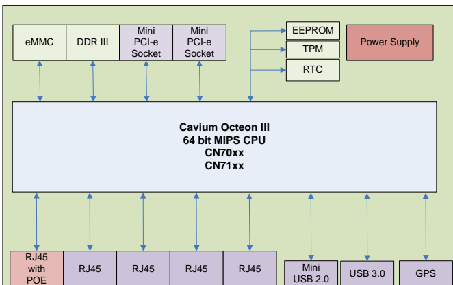
Block Diagram of Tahoe 8720
