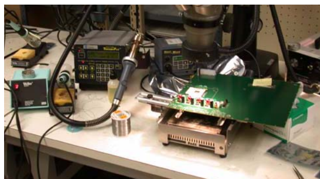
FIGURE 6. HOT PLATE REWORK STATION OVERVIEW
