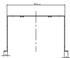
Front view AH96 for the UMG 96RM
