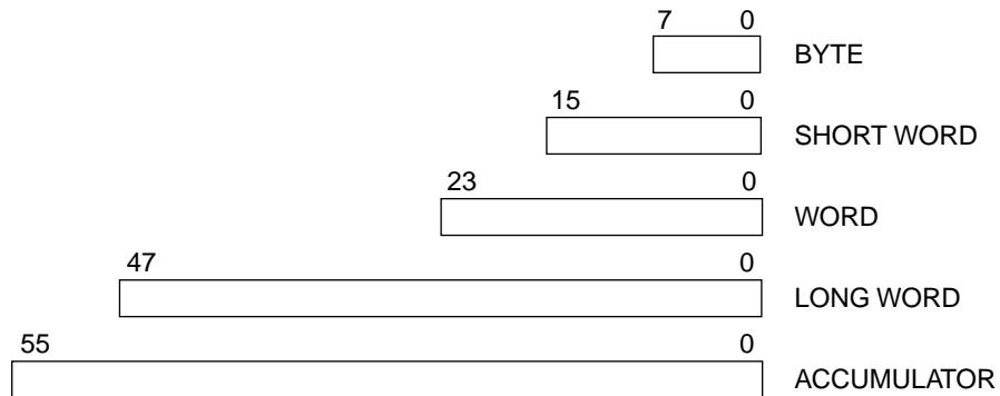
Figure 6-3 Operand Sizes
