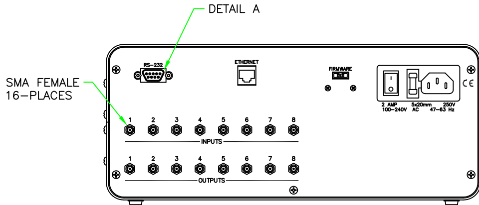
REAR VIEW
