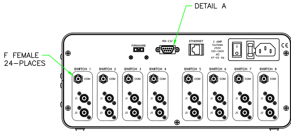
REAR VIEW
