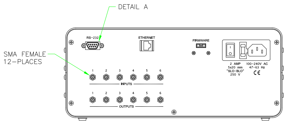
REAR VIEW
