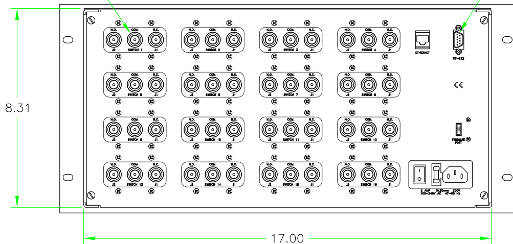
REAR VIEW
