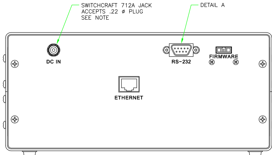
REAR VIEW
