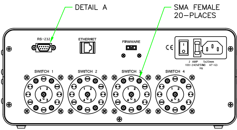
REAR VIEW
