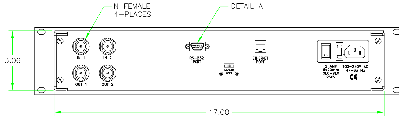
REAR VIEW
