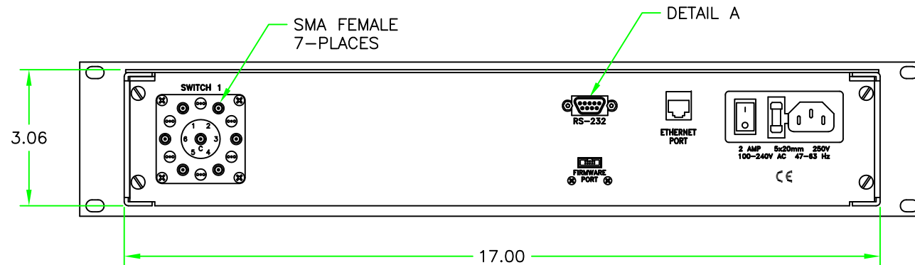
REAR VIEW
