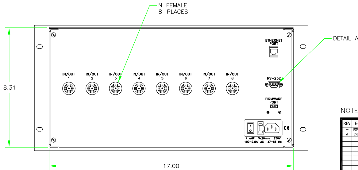
REAR VIEW
