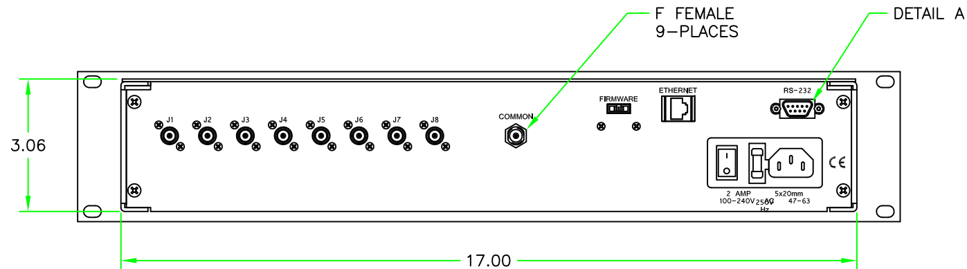
REAR VIEW
