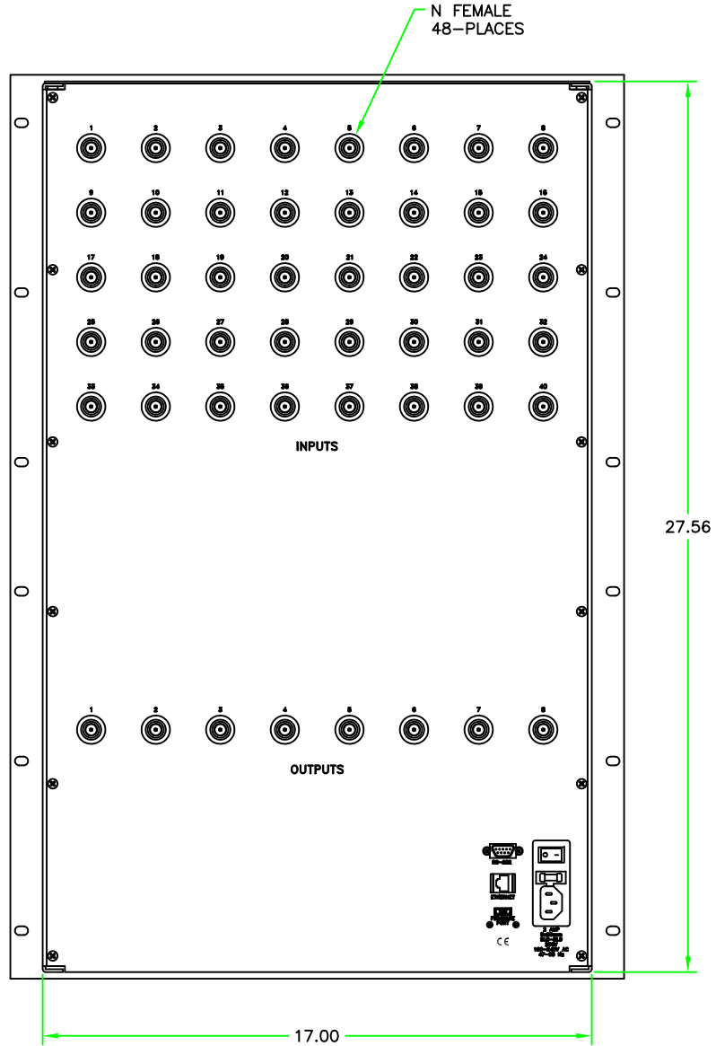
REAR VIEW
