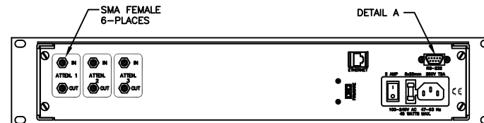
-03 (i.e. 3 ATTENUATORS)
