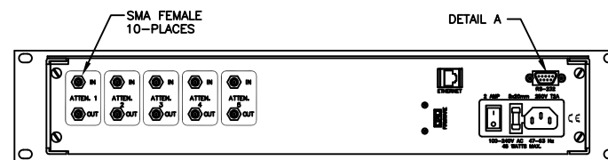
-05 (i.e. 5 ATTENUATORS)
