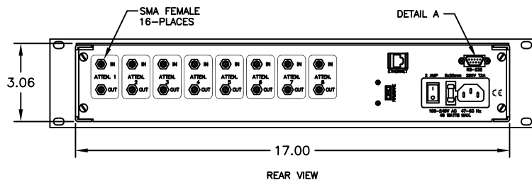
-08 (i.e. 8 ATTENUATORS)
