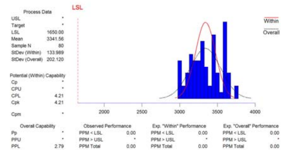
Process Capability Analysis for Sn63 NC Soldmask w/Slot
