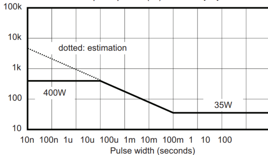
Pulse peak power (W) - 0.01 Duty Cycle
