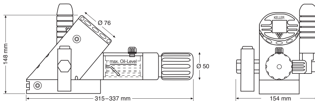
High Pressure Calibrator Outline Drawing
