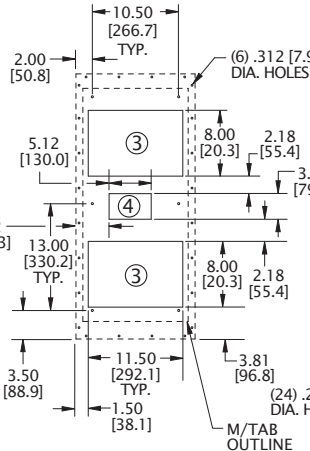
MOUNTING PLAN M/TAB & CUTOUTS
