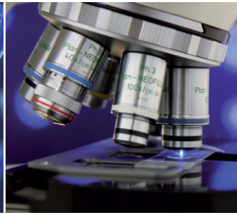
Multi-photon microscopy
