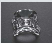
FLARE-C 29.0 MM X 24.5 MM X 14.5 MM PMMA
