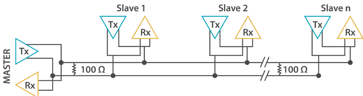
Figure : Multi-drop Network connection
