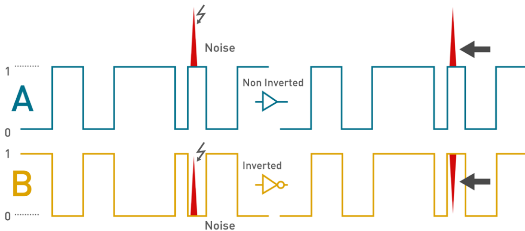
Figure : Differential signaling operation
