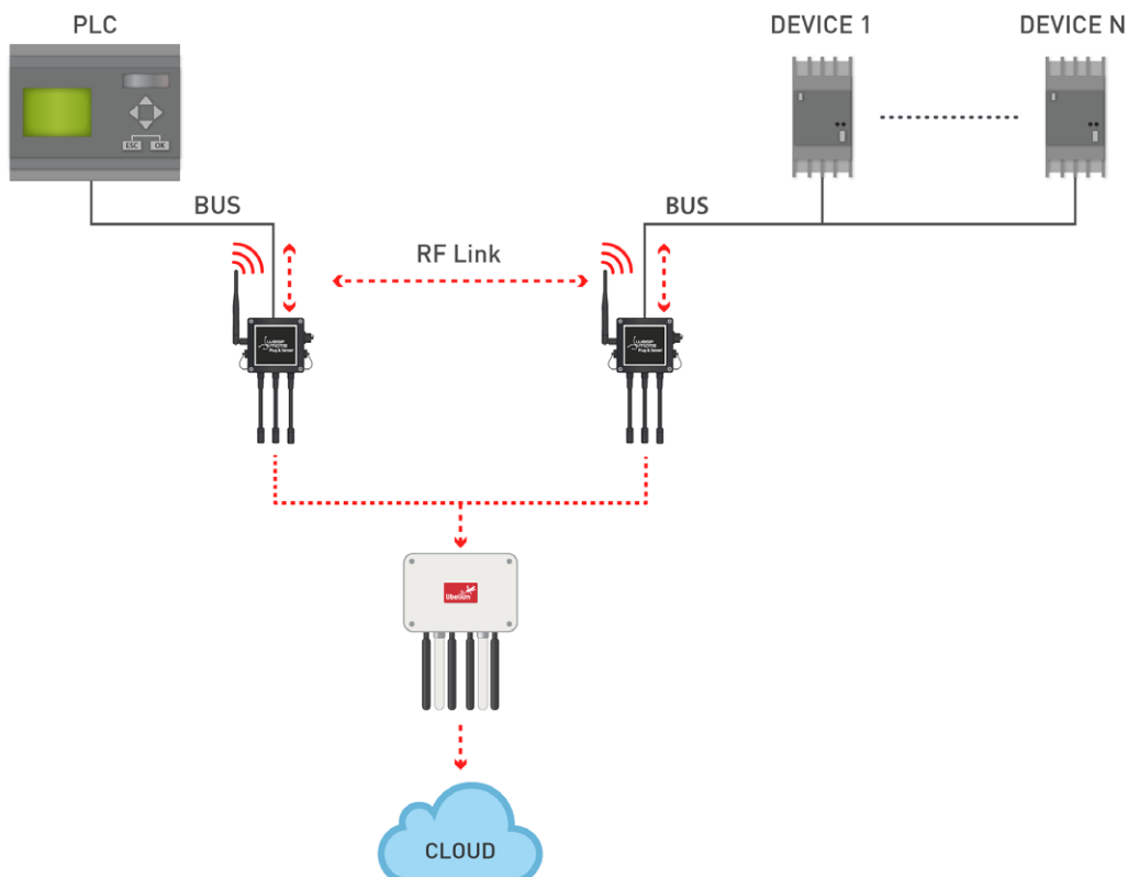
Figure : Waspote replacing wired connections
