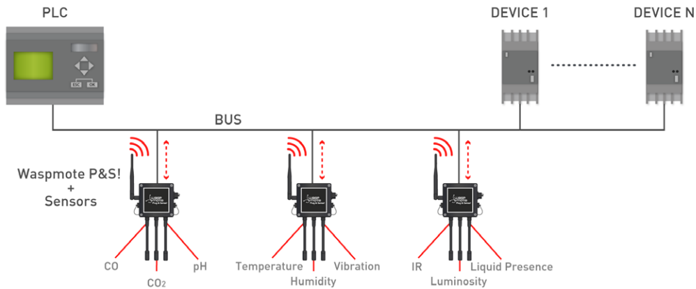
Figure : Waspote integrated in an RS-485 network
