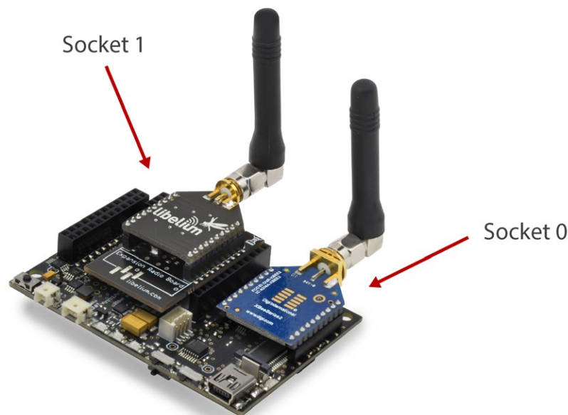
Figure : Waspote with XBee radio on socket0 and WiFi module on socket 1
