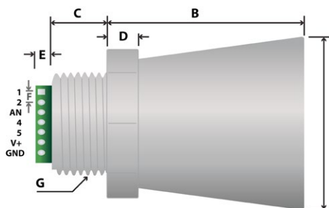
Figure: Ultrasonic I2CXL-MaxSonar®-MB7040 sensor dimensions
