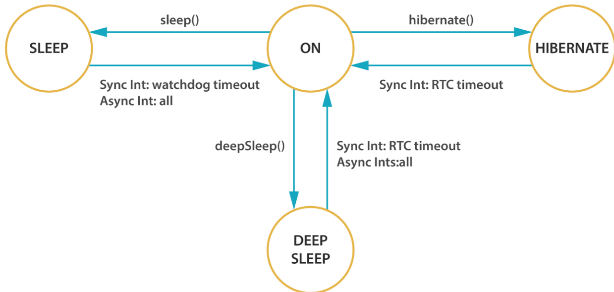
Figure: Diagram of mode in Waspote
