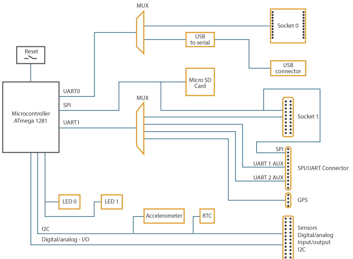
Figure: Waspote block diagrams – Data signals
