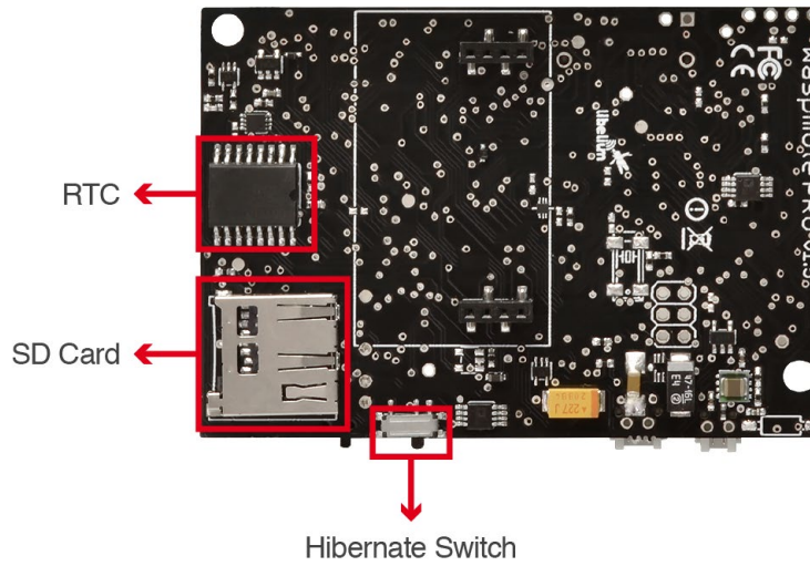
Main Waspote components – Bottom side
