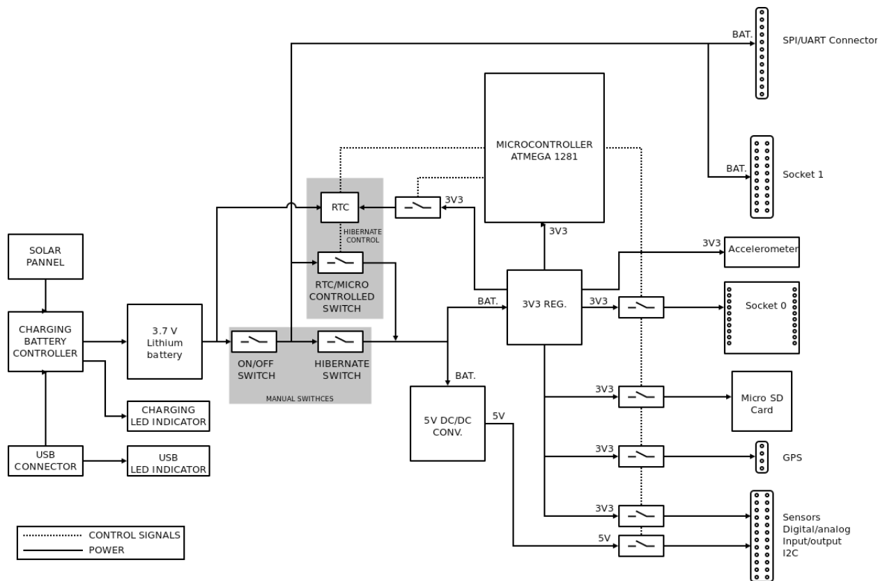
Figure: Wasp mote block diagrams – Power signals
