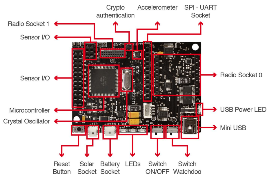
Figure: Main Waspote components – Top side
