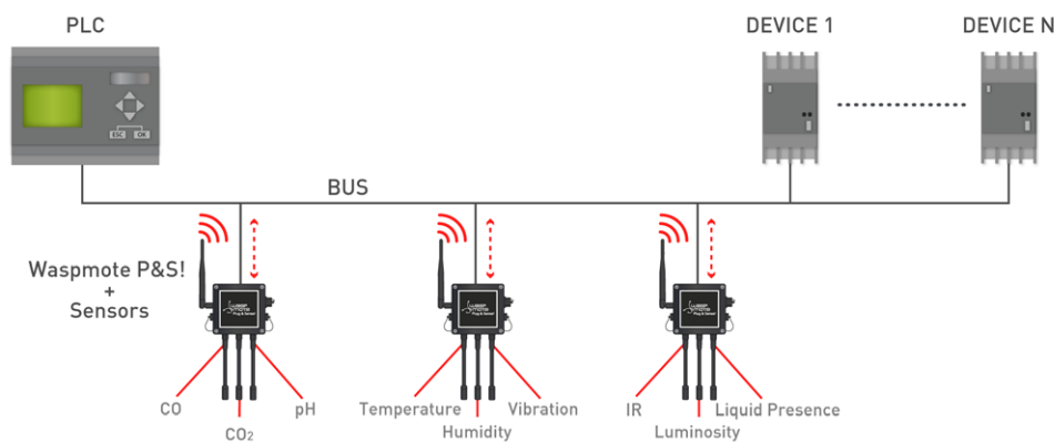
Figure: Module in wireless sensor network applications
