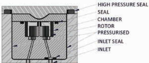
Figure 3 Pressure Balanced Chamber design
