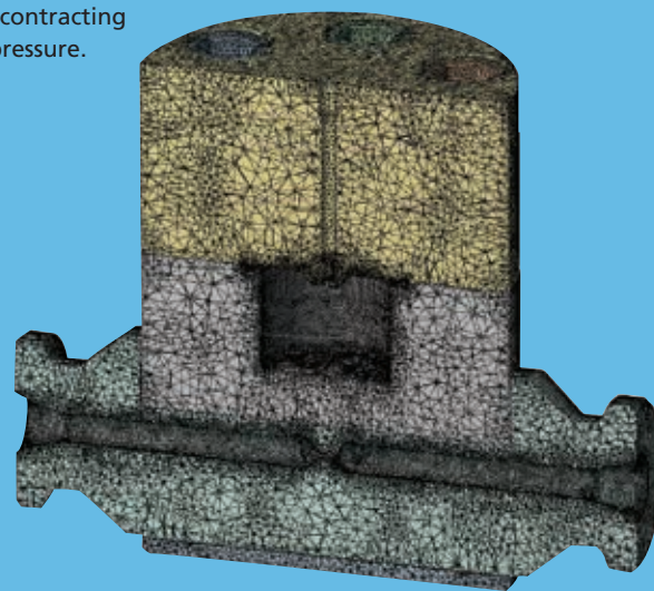
Figure 2 FEA mesh analysis of a 1035bar VFF
