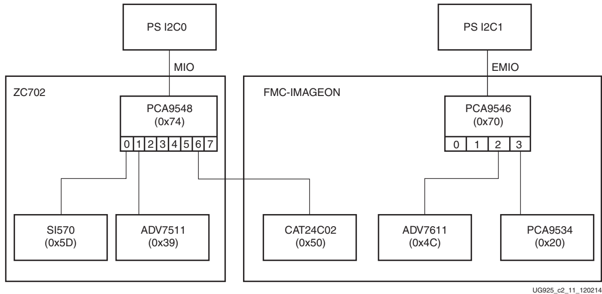
Figure 2-2: I2C Sub-system
