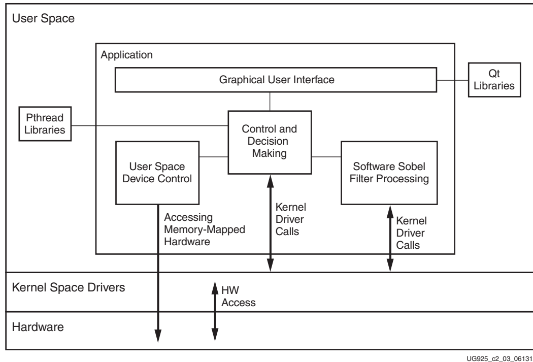
Figure 2-6: Application Functional Blocks
