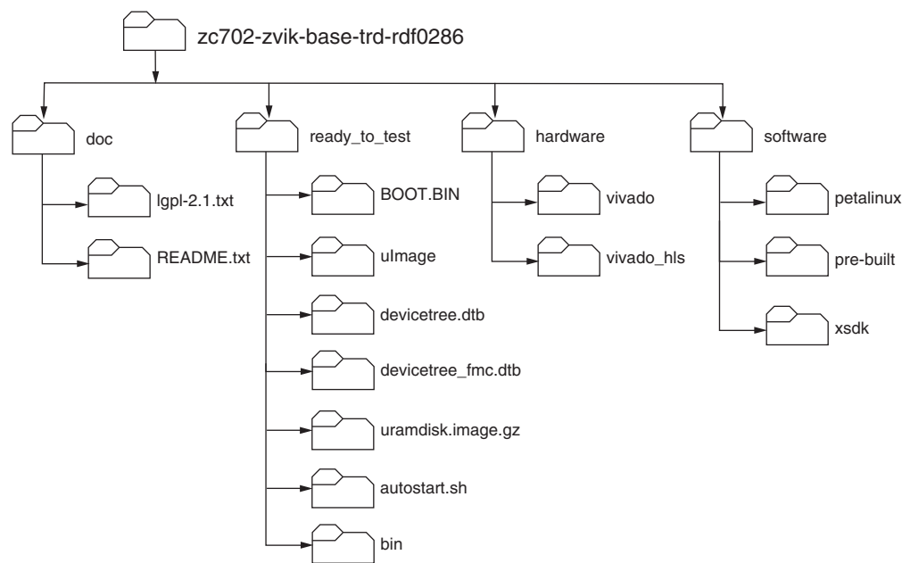
Figure C-1: Directory Structure
