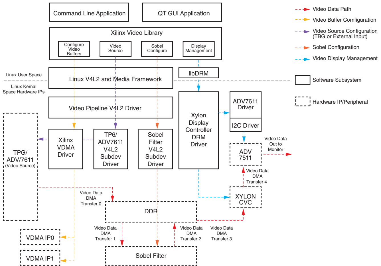
Figure 2-4: Software Schematic
