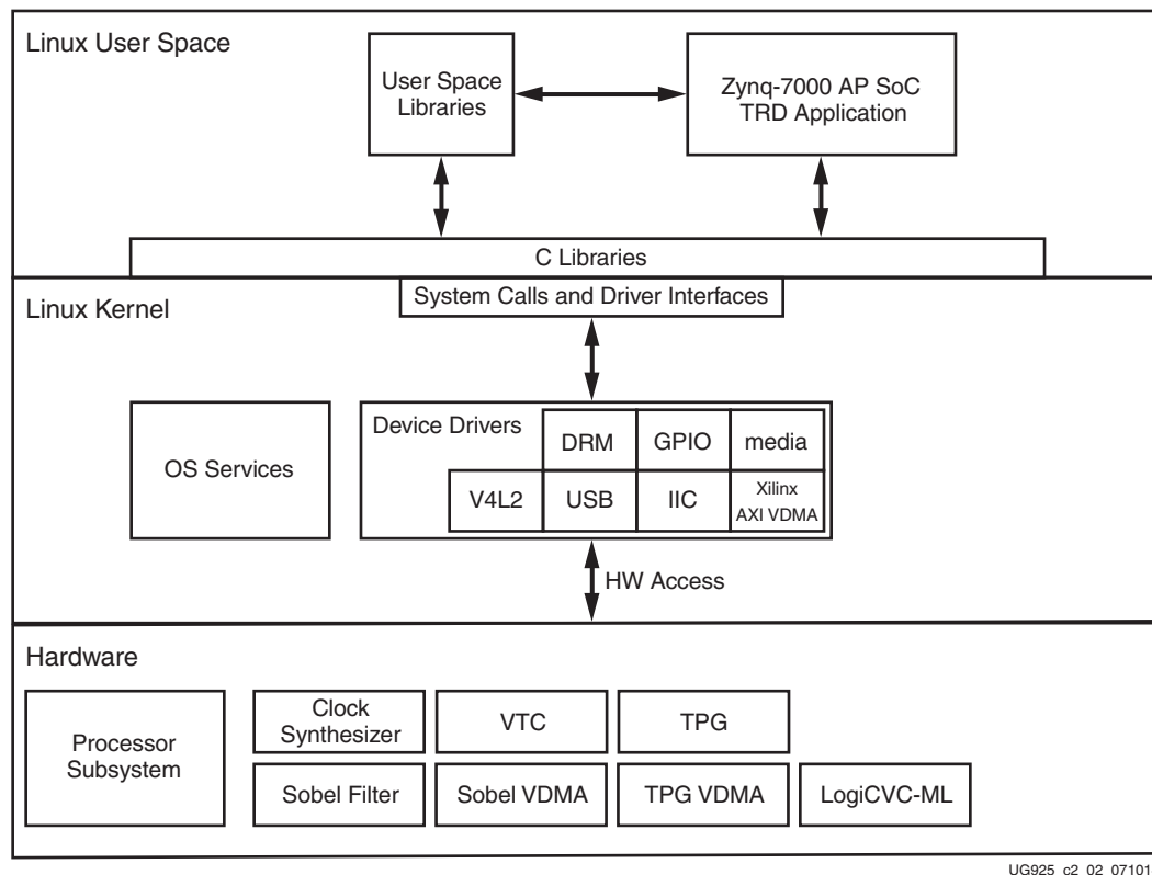
Figure 2-5: Software Architecture: Top Level View
