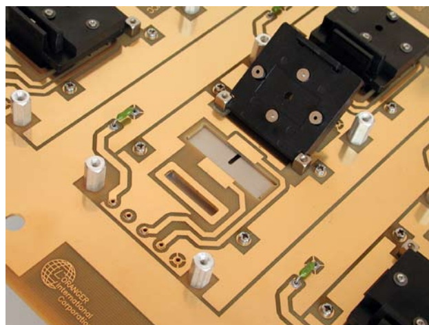
High Frequency Board and Sockets
