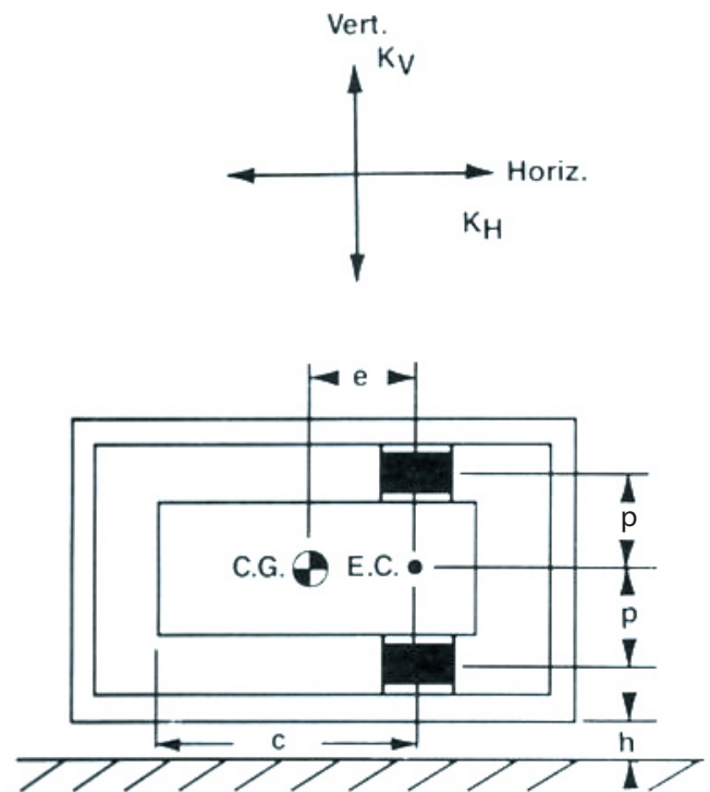
FIGURE 37 – COUPLED FLAT SIDE DROP
