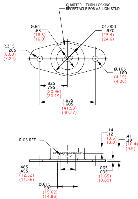
FIGURE 1 – PART DIMENSIONS
