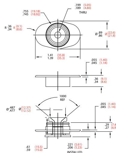
FIGURE 2 – J-23436-8 PART DIMENSIONS
