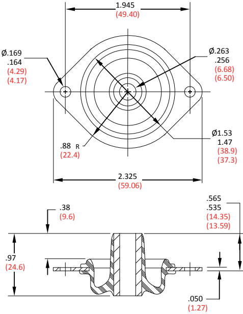
FIGURE 1 – PART DIMENSIONS
