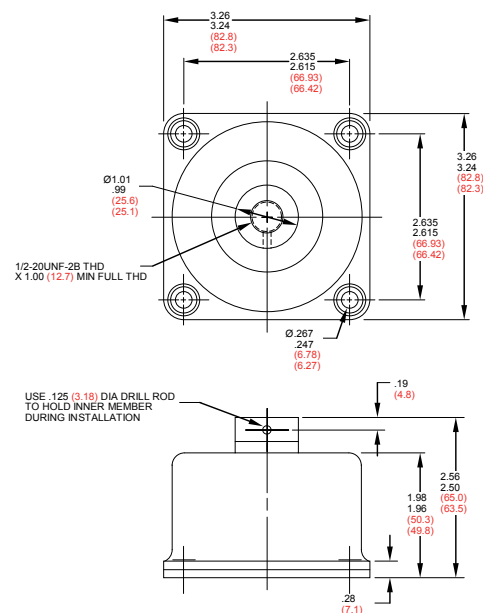
FIGURE 1 – HTC SERIES PART DIMENSIONS
