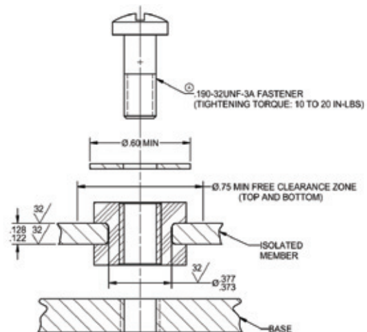
FIGURE 3 – CB-1077-52 INSTALLATION DRAWING
