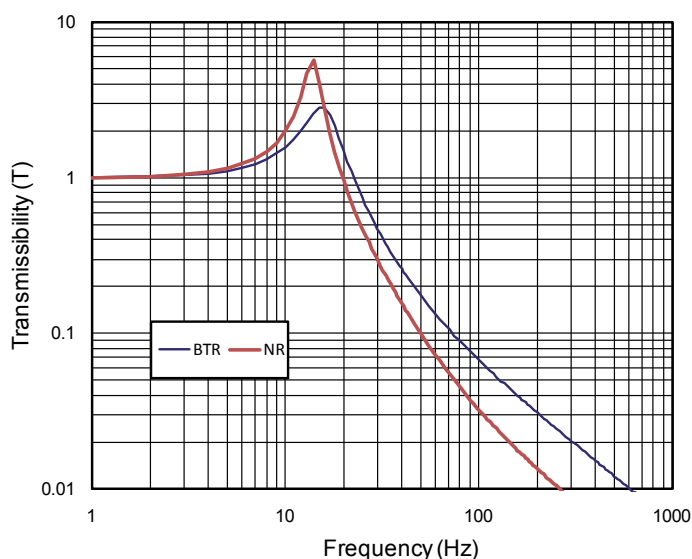
FIGURE 4 – TRANSMISSIBILITY VS. FREQUENCY
