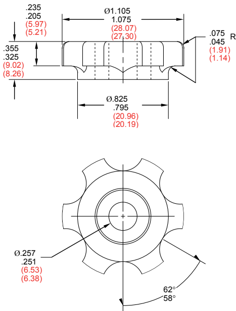
FIGURE 1 – PART DIMENSIONS
