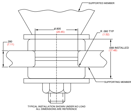
FIGURE 2 – INSTALLATION DRAWING
