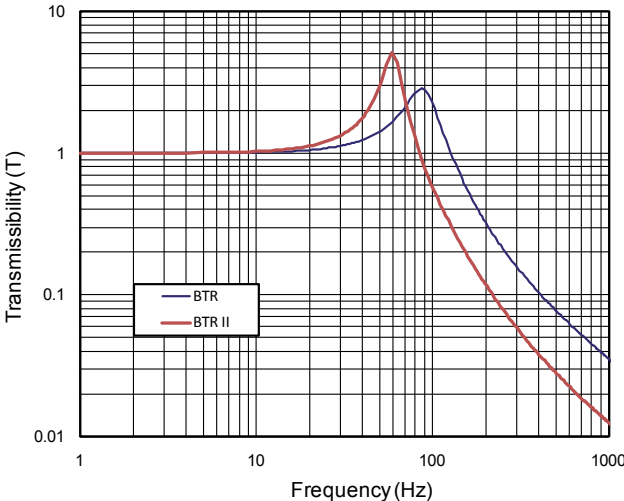
FIGURE 2 – TRANSMISSIBILITY VS. FREQUENCY
