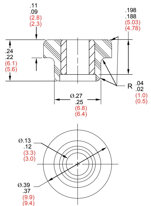
FIGURE 1 – PART DIMENSIONS
