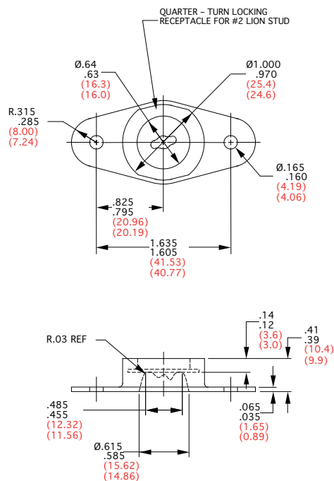
FIGURE 1 – PART DIMENSIONS
