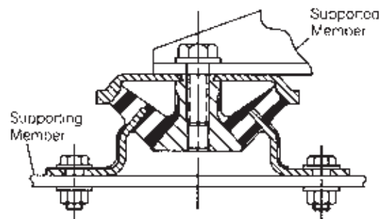
FIGURE 1 – TYPICAL INSTALLATION
