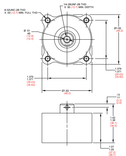
FIGURE 2 – UT1 SERIES PART DIMENSIONS
