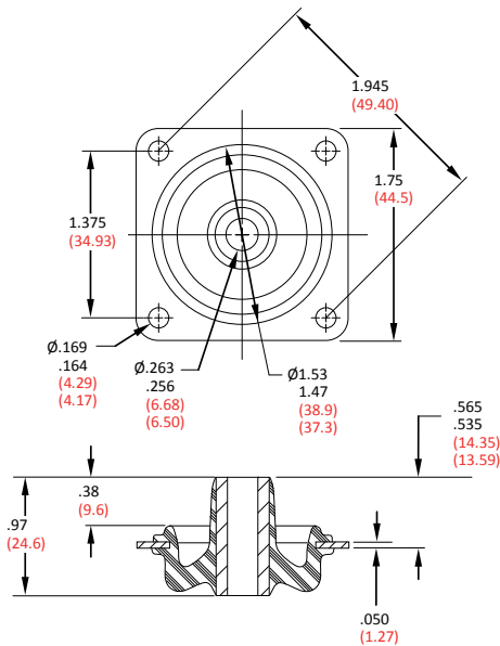
FIGURE 1 – PART DIMENSIONS
