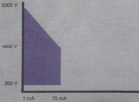
Output Voltage Compliance Chart, HVS Series Stations and Sources
