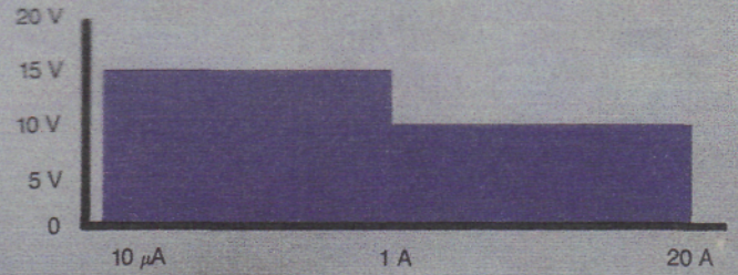
Mainframe Collector Current Supply Compliance Chart
