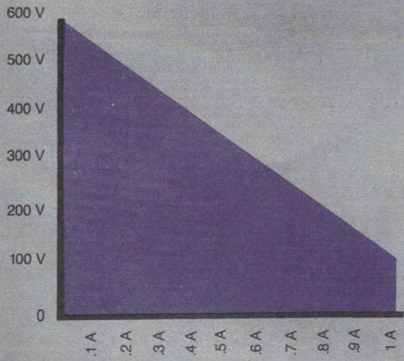
Mainframe High Voltage Supply Compliance Chart. The extended operation area is available as a hardware option.
