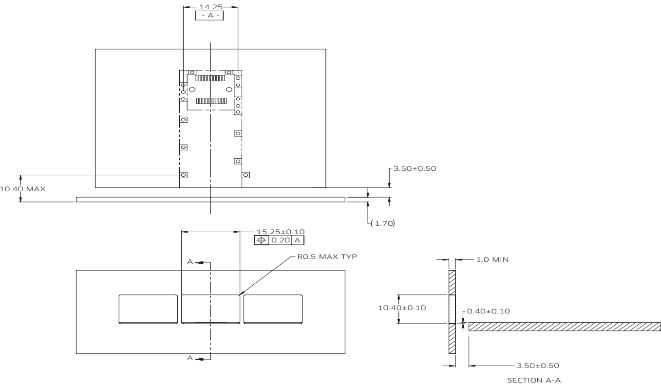
Figure 4 Recommended panel cut-out and PCB offset
