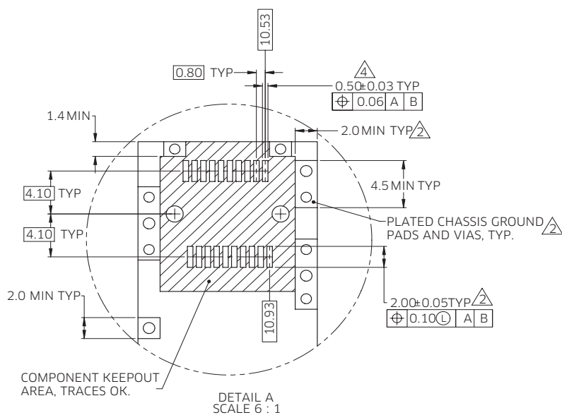
Figure 2 Board layout
