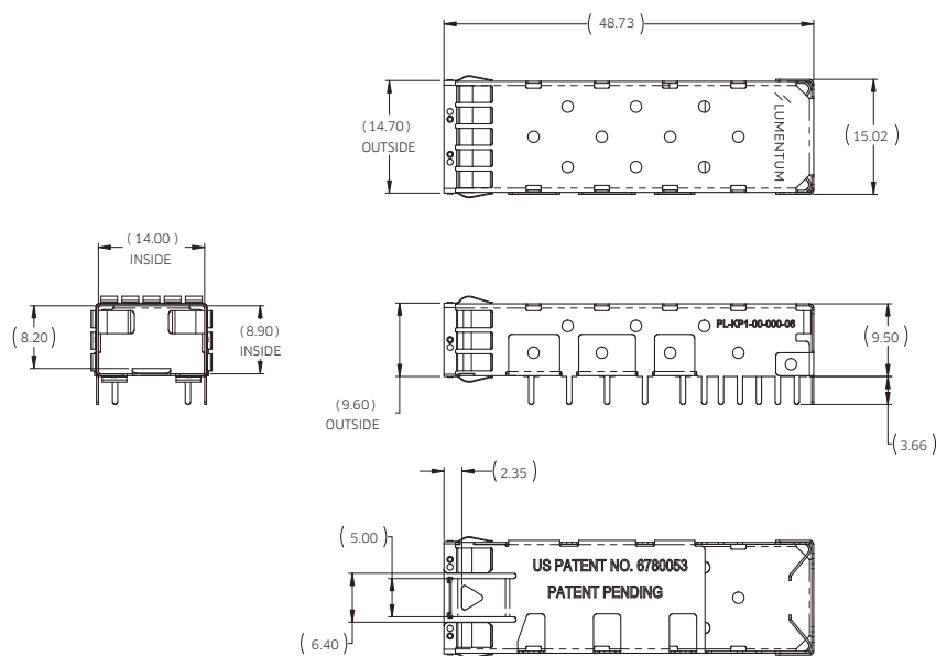
Figure 1 Standard solder-down cage mechanical drawing (PL-KP1-00-000-06)
