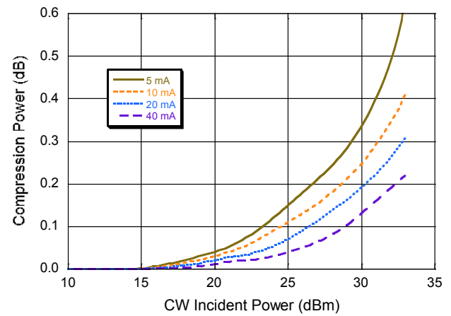
Compression Power
