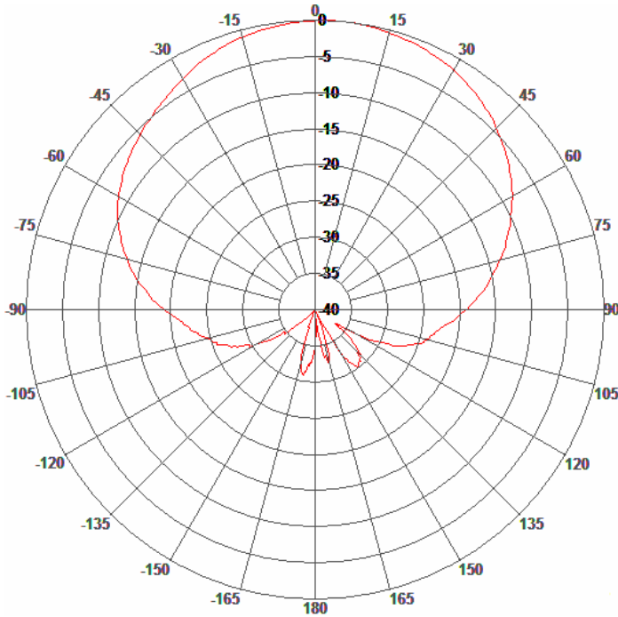
E-Plane Patterns
