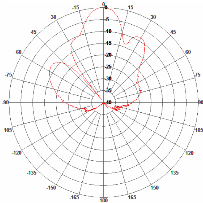
E-Plane Pattern
