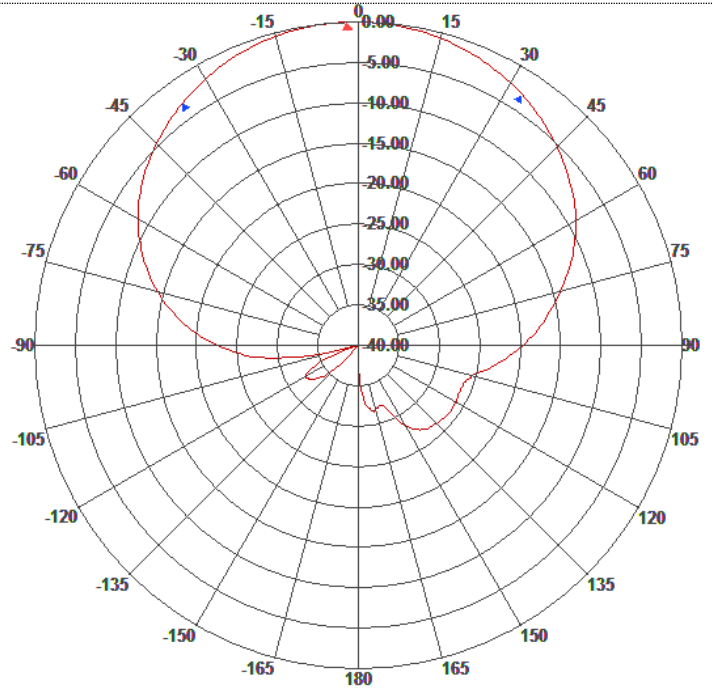
Azimuth Pattern
